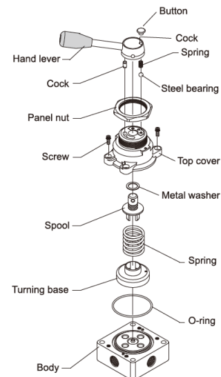
Model: TSV30043-02, 03, 04
