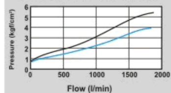
Model: TSV30043-02, 03, 04
